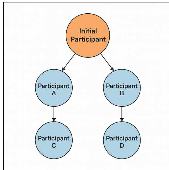
Figure 2: Snowball Sampling.
